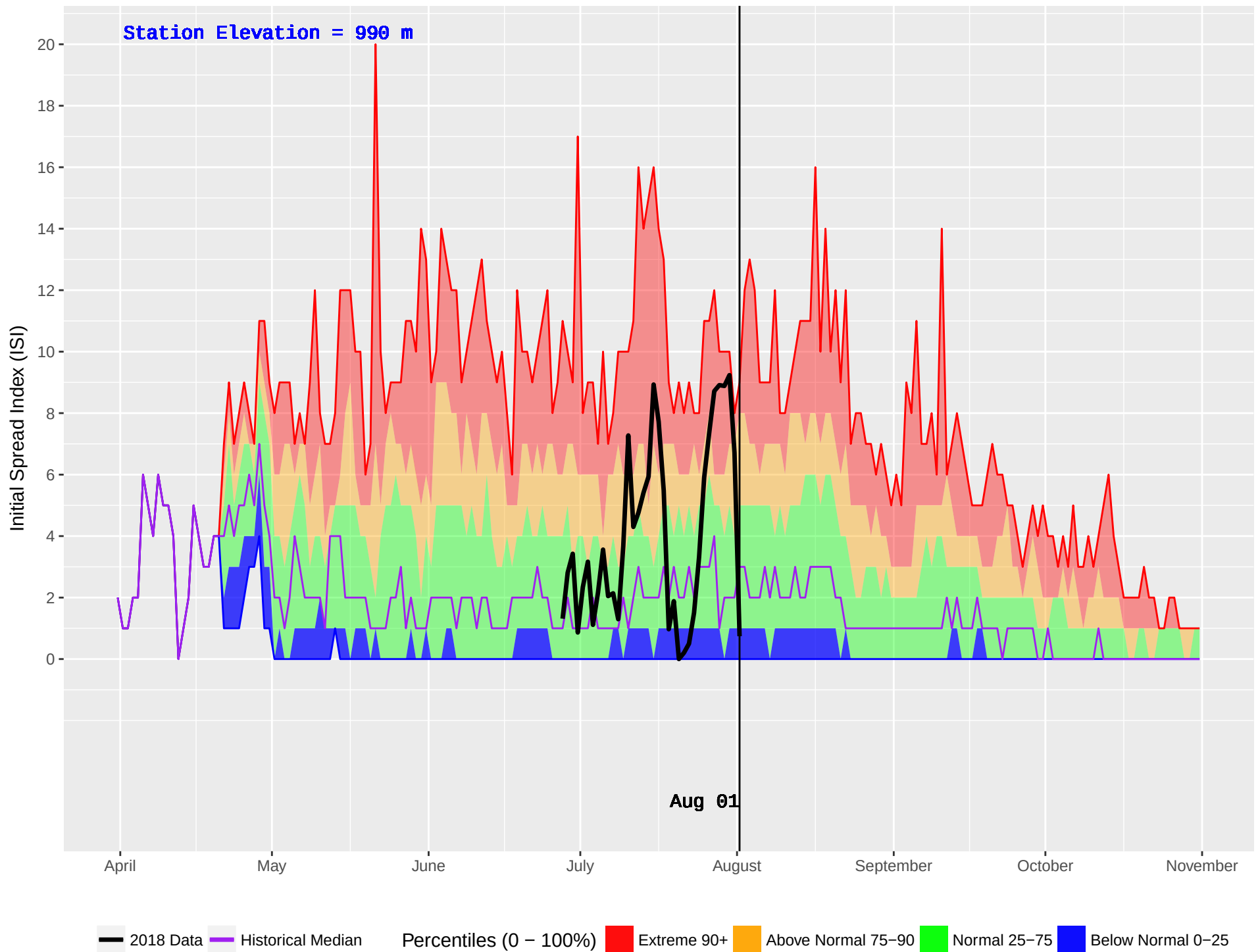
LOVELL COVE (163) : Historical (1979–2016) and Current (2018) Daily Initial Spread Index (ISI)
